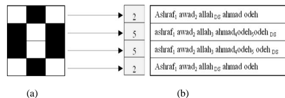
Fig. 1: (a): Binary image watermark and its decimal equivalent vector, (b): Watermarking example; where subscripts represent space number and DS corresponds to double space
