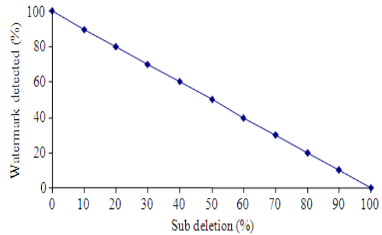
Fig. 3: Robustness results due to the 'subset deletion attack'
