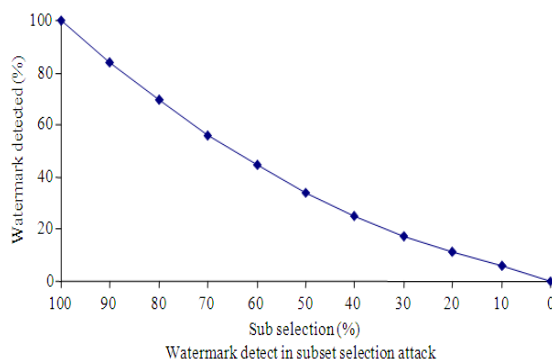
Fig. 6: Robustness results due to the 'subset selection attack'
