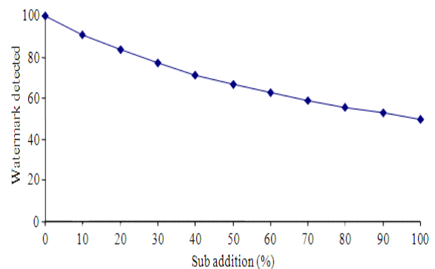
Fig. 4: Robustness results due to the 'subset addition attack'
