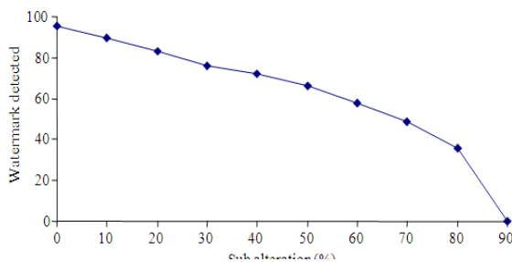
Fig. 5: Robustness results due to the 'subset alteration attack'
